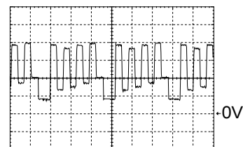
③ 1V/cm, 20μs/cm
